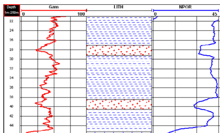
Example neutron porosity log (NPOR)
